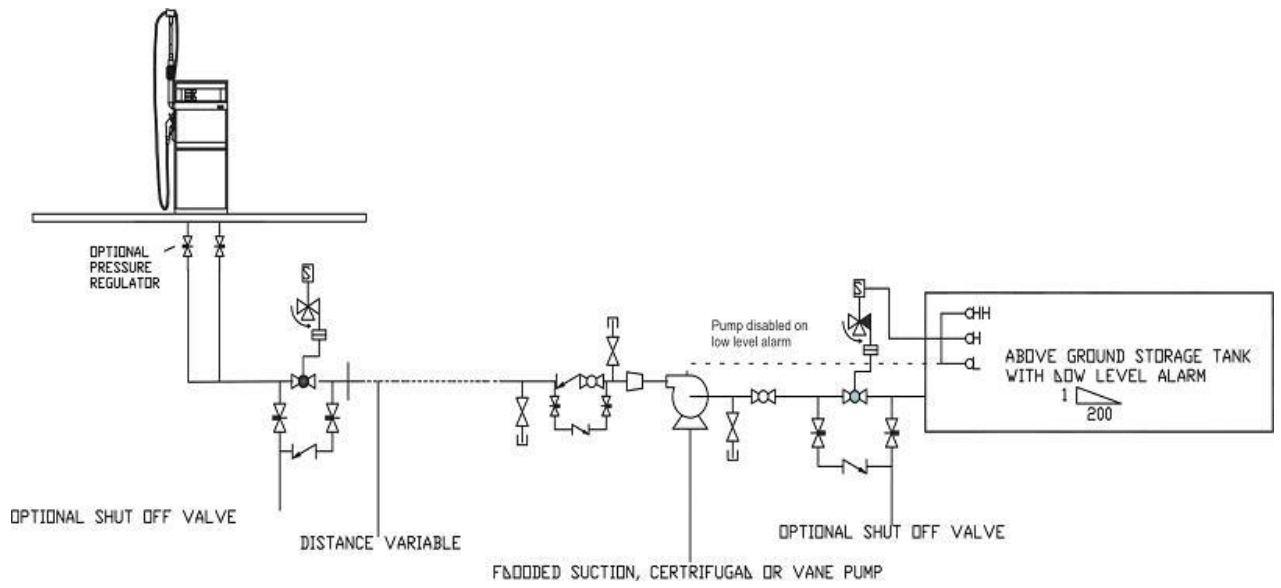
With External Pump and Above-ground Supply Tank – Variant 3
