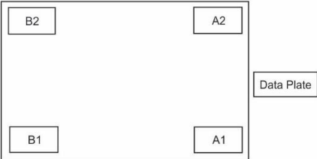
MR or MMR housing, Quad Hose model (MMA30-160SQ; MMA30-80SQ; MMA30-40SQ)
